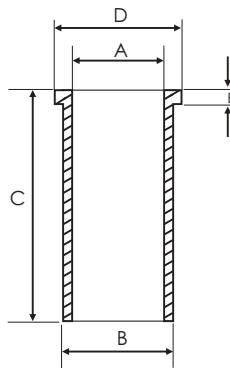
WITH FLANGE
