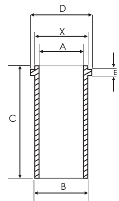
WITH FLANGE & FIRE LIP
